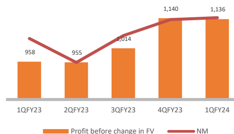
PBCFV (Rs'mn) vs Net Margin
